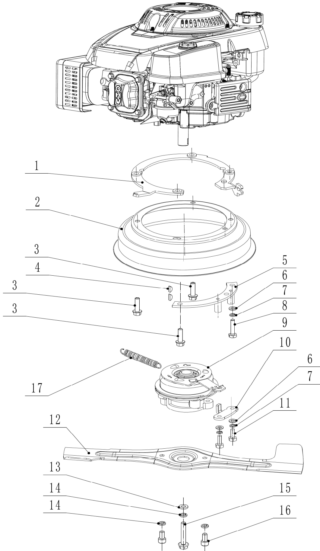
Blade components
